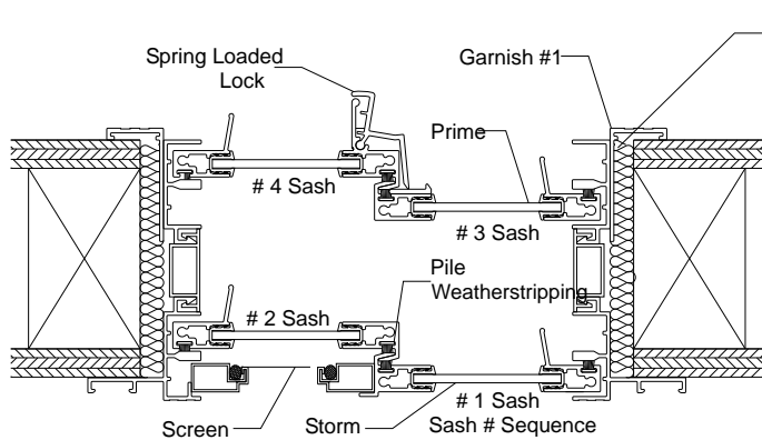
3376 Vertical Section
