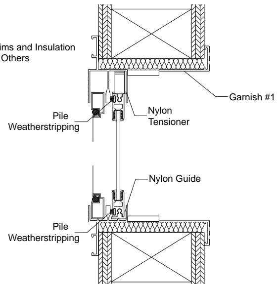
Mark IV Horizontal Section
