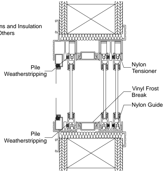
3376 Horizontal Section
