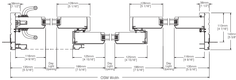
3-LITE HORIZONTAL SECTION
