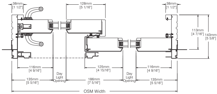
HORIZONTAL SECTION
