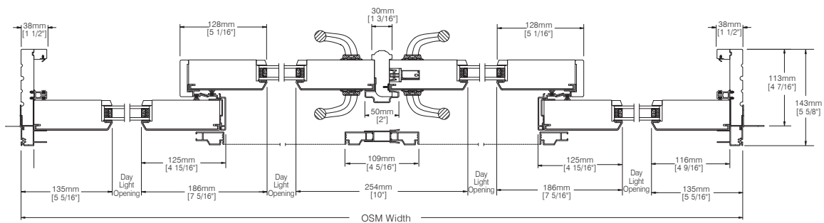
4-LITE HORIZONTAL SECTION
