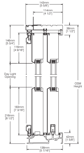
VERTICAL SECTION
