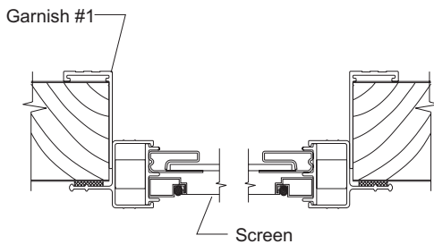
8000 Horizontal Section
