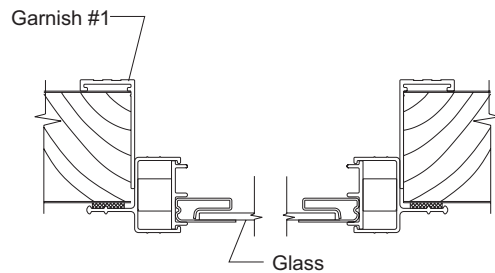
8000 Horizontal Section
