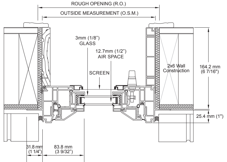
260 CASEMENT HORIZONTAL SECTION
