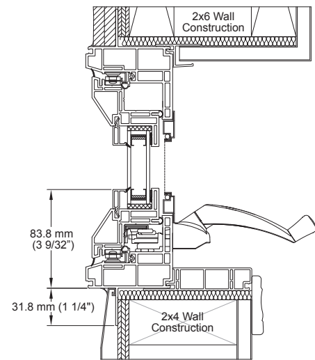
260 CASEMENT VERTICAL SECTION
