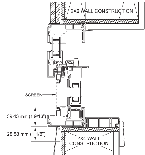
135 SINGLE HUNG VERTICAL SECTION
