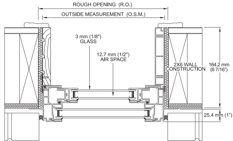
135 SINGLE HUNG HORIZONTAL SECTION
