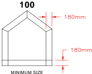
100 MINIMUM SIZE 410mm W x 410mm H MAXIMUM SIZE - NARROW BAR 1500mm W x 1800mm H MAXIMUM SIZE - WIDE BAR 1800mm W x 2020mm H
