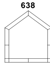
638 MINIMUM SIZE 410mm W x 410mm H MAXIMUM SIZE - NARROW BAR 1800mm W x 2000mm H MAXIMUM SIZE - WIDE BAR 2400mm W x 2100mm H
