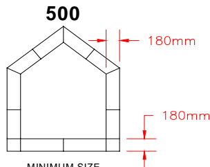
500 MINIMUM SIZE 410mm W x 410mm H MAXIMUM SIZE - NARROW BAR 1800mm W x 2000mm H MAXIMUM SIZE - WIDE BAR 2400mm W x 2100mm H
