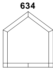
634 MINIMUM SIZE 410mm W x 410mm H MAXIMUM SIZE - NARROW BAR 1800mm W x 1800mm H MAXIMUM SIZE - WIDE BAR 2400mm W x 2020mm H
