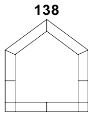
138 MINIMUM SIZE 410mm W x 410mm H MAXIMUM SIZE - NARROW BAR 1800mm W x 2000mm H MAXIMUM SIZE - WIDE BAR 2400mm W x 2100mm H
