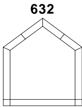
632 MINIMUM SIZE 410mm W x 410mm H MAXIMUM SIZE - NARROW BAR 1500mm W x 2000mm H MAXIMUM SIZE - WIDE BAR 1800mm W x 2400mm H
