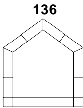
136 MINIMUM SIZE 410mm W x 410mm H MAXIMUM SIZE - NARROW BAR 1500mm W x 2000mm H MAXIMUM SIZE - WIDE BAR 1800mm W x 2400mm H
