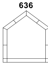
636 MINIMUM SIZE 410mm W x 410mm H MAXIMUM SIZE - NARROW BAR 1500mm W x 2000mm H MAXIMUM SIZE - WIDE BAR 1800mm W x 2400mm H
