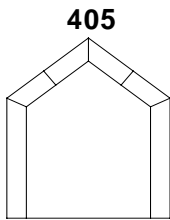
405 MINIMUM SIZE 410mm W x 410mm H MAXIMUM SIZE - NARROW BAR 1800mm W x 1800mm H MAXIMUM SIZE - WIDE BAR 2400mm W x 1800mm H
