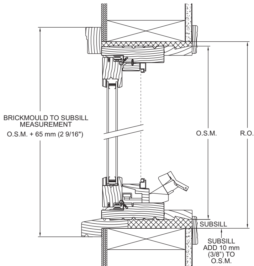
525 CASEMENT VERTICAL SECTION
