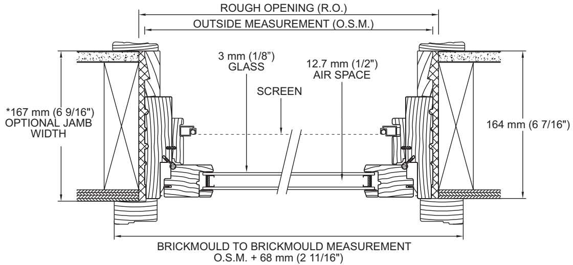
525 CASEMENT HORIZONTAL SECTION
